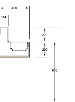
DfE4 Thermo Profile Thermoformed trough with wall mounted taps. A choice of brackets or underframe.
