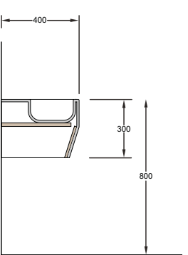
DfE3 Thermo Profile Thermoformed trough with wall mounted taps.
