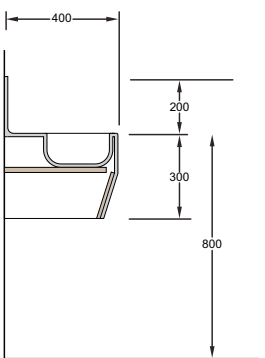
DfE2 Thermo Profile Thermoformed trough with deck mounted taps.
