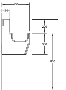
DfE1 Thermo Profile Thermoformed trough with wall mounted taps.
